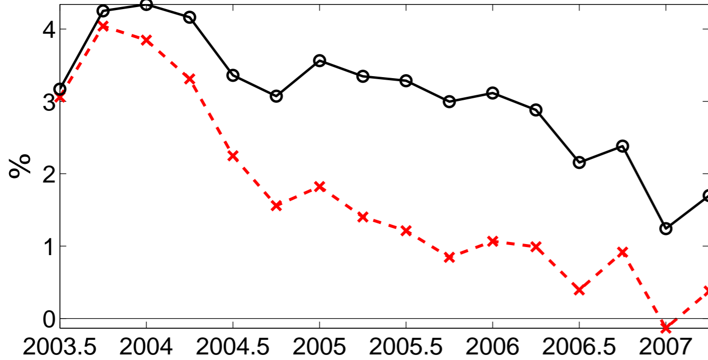
Four-Quarter Output Growth
